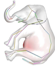
Figure 11: Example of weight distribution in a complex case. The bulging in the belly parts depends on the distance to the spine. To give nicer results, the distances to the bones of the legs are not taken into account.
