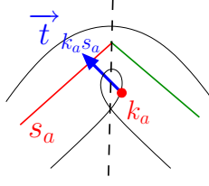
Figure 7: Method to avoid self-intersection. Vertex k_a is detected in the region linked to the green bone while its original region was the red one. k_a is thus translated along \mathbf{t}_{k_a s_a} until it reaches border of its associated region.
