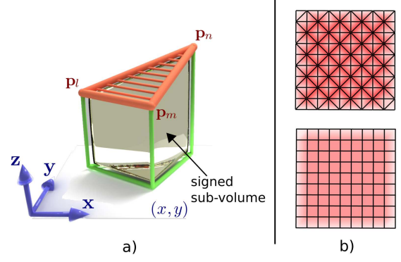
Figure 2: a) Prism obtained by projecting the triangle (\mathbf{p}_l, \mathbf{p}_m, \mathbf{p}_n) onto the (x, y) plane. The summation of all the signed sub-volumes give the interior volume of the triangular mesh. b) Color encoding of \|\nabla V\| over a triangulated quad-mesh (top) using differentiation of eq. 1, and using eq. 2 directly on the bilinear patches (down). Note the periodical pattern appearing in the first case due to the change of valence.
