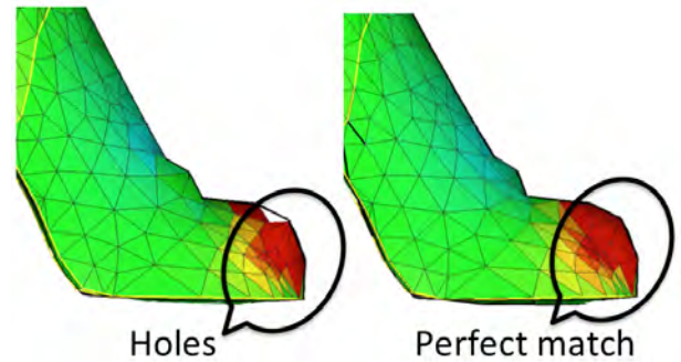
Fig. 6. Constraining isolated vertices to match the silhouette may lead to incomplete silhouettes (left) while our edge based approach ensures perfect silhouette match.
