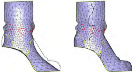
Fig. 9. Silhouette matching: Projection of most protruding edges to the silhouette and mesh deformation best preserving normals. The silhouettes strokes of the side-view are perfectly matched, as well as the 3D feature line constraints (yellow). The mesh edges marked in black on the bootleg are the selected edges tied to the silhouette stroke of the front view.
