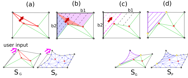
Fig. 7. Generation of rulings to favor further bending when the propagation reaches the boundary \partial S at both ends. (a) The triangle of maximal compression is in red. (b) Propagation of triangle strip with imaginary rulings as dashed lines. Both borders belong to \partial S . (c) Rulings inserted (purple lines). (d) Final meshing of \bar{S} and S_G .
