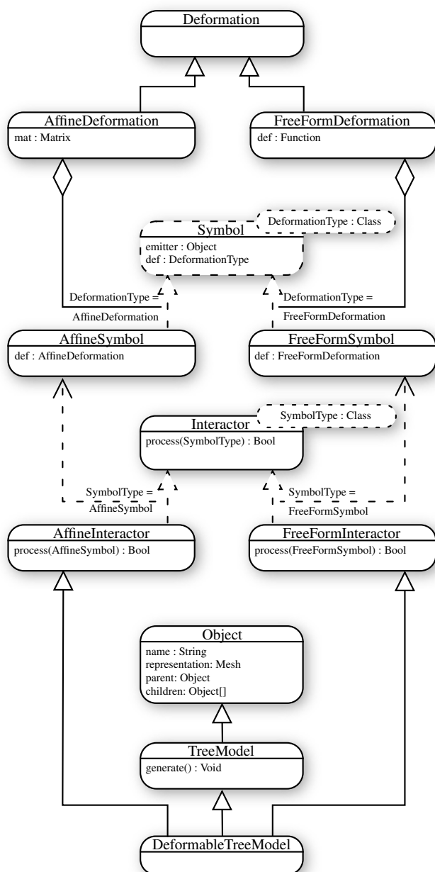
Figure 13: UML class diagram of our C++ implementation of deformation grammars through interactors. According to standard UML notations: \longrightarrow stands for inheritance; \cdots \rightharpoonup stands for dependency; \cdots \triangleright stands for realization; And \longrightarrow \diamond stands for aggregation.
