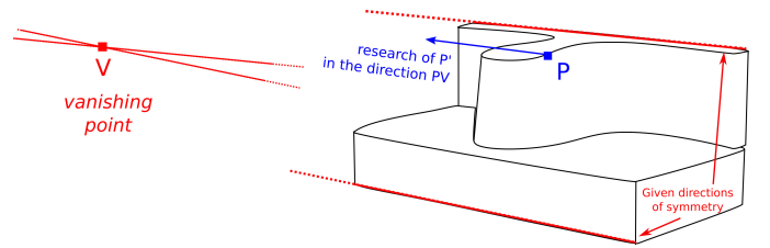
Figure 14: Finding the vanishing point of the image from two annotated red lines would improve the search for the point symmetric to P.
