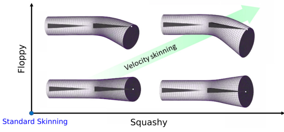
Figure 3: The deformer of squashy and floppy velocity skinning reveal information in the still about the speed and direction of the motion that is not visible in the standard skinning surface.
