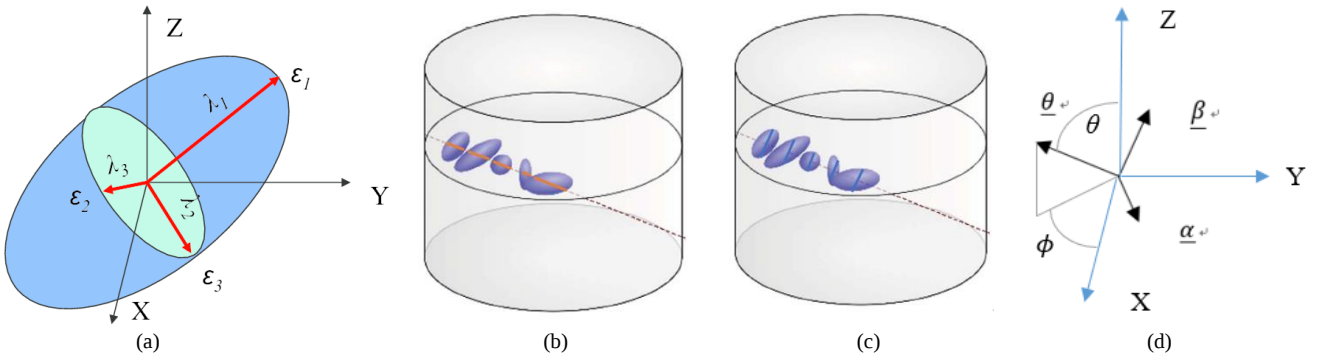
Fig. 1. (a) A second rank tensor illustrated as an ellipsoid. The eigenvectors \underline{\epsilon}_1, \underline{\epsilon}_2, \underline{\epsilon}_3 of the tensor are the 3-unit vectors along the principal semi-axes of the ellipsoid, and the eigenvalues \lambda_1, \lambda_2, \lambda_3 are the lengths of the principal semi-axes. (Drawn based on Fig. 5 in [46]) (b) p_{\underline{\theta}}^{\underline{\theta}\underline{\theta}} and (c) p_{\underline{\theta}}^{\underline{\beta}\underline{\beta}} are the integrals along \underline{\theta} of the orange intersections (along \underline{\theta} ) and blue intersections (along \underline{\beta} ), respectively. Here the integration line goes through the centers of all ellipsoids. (Drawn based on Fig. 5 in [46] but modified to indicate the tensor measurements along \underline{\theta} and \underline{\beta} .) (d) Illustrations of the three orthogonal vectors \underline{\theta}, \underline{\alpha}, \underline{\beta} , zenith angle \theta and azimuth angle \phi .
