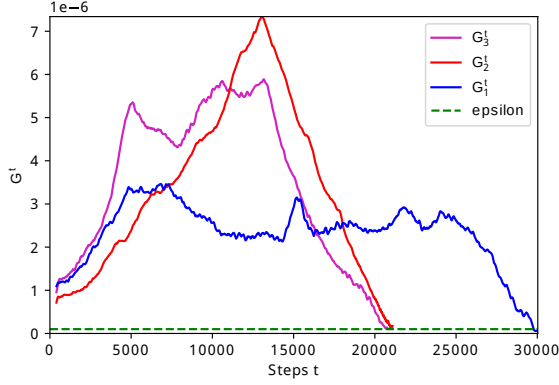
Figure 13: \mathcal{G}' for the three stress oriented structures of the chair
