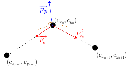
Fig. 4: Force due to pressure (in blue) and forces due to elasticity (in red) on a discrete position (middle black dot). Each position has two neighbors in which the forces of elasticity are directed.
