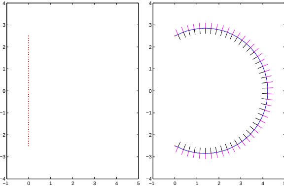
Fig. 18: Numerical validation of the circle solution for an initial position with vanishing second derivative. The picture on the left shows the initial position of the membrane making a straight line from the first to the last point. The picture on the right is the final shape after dilatation. This shape has converged to a portion of a circle.
