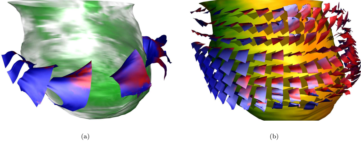
Figure 15: Figure (a) shows some large color coded sheets around the left ventricular positioned in the basal region. The color of the sheet encodes the z component of the fiber direction (the blue intensity is for a planar fiber and red for a fiber going up or down). Some noise can be seen in the epicardium. The color of the endocardium encodes the z component of the sheet normal. The green color indicates a large z component, meaning that the sheet is almost in the radial plane of the ventricle. At the opposite, the white transparent color indicates a normal directed more perpendicular to e_z , in these regions, sheets are less planar. The seeding of small sheets on the left ventricle is represented in Figure (b). The spatial variation of the orientation of these surfaces is shown. The color encoding on the surface is the same as in (a). Some regions can be differentiated where the cleavage planes fit well to the model crossing the wall and some other are far more vertical. The global structure is therefore complex. The color of the endocardium is the first and second component of the fiber. Thus, the rotation of the fiber structure around the endocardium can be seen.
