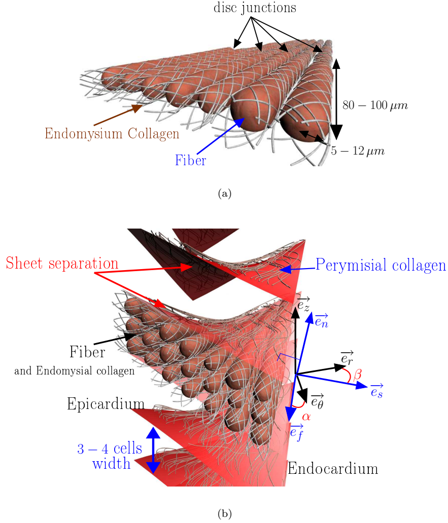
Figure 2: Figure (a) shows the geometry of the fiber and endomysial collagen in the heart. The long oval structures correspond to the fibers. Figure (b) shows the lamina structure with the cylindrical basis ( \mathbf{e}_r, \mathbf{e}_\theta, \mathbf{e}_z ) and the sheet basis ( \mathbf{e}_f, \mathbf{e}_s, \mathbf{e}_n ).
