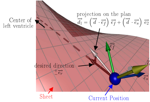
Figure 5: Projection of the desired radial direction \mathbf{e}_r (this direction is shown by the dashed lines) onto the sheet surface defined by the normal \mathbf{e}_n . The vector \mathbf{e}_f defines the fiber direction and \mathbf{e}_s defines the sheet direction. \mathbf{e}_n is the normal to the surface and \mathbf{d}_1 is the projection of \mathbf{e}_r onto the plane spanned by the vectors \mathbf{e}_f and \mathbf{e}_s .
