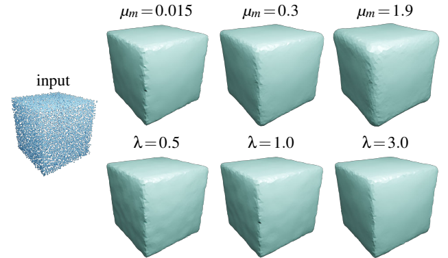
Figure 9: Effects of parameters: On a simple noisy cube example (Gaussian noise with a standard deviation equal to 1% of the model diameter), running our minimization with varying values of the selectivity \mu_m captures (left) or do not capture (right) the sharp edges (top); if the smoothness strength \lambda is changed, the result ends up with more or less flat faces (bottom). We used \lambda = 3.0 for the top row, and \mu_m = 0.13 for the bottom row.
