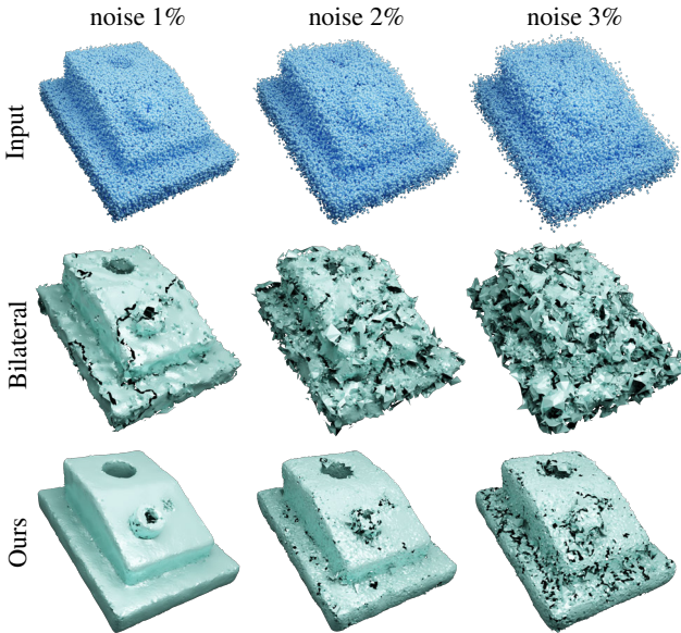
Figure 13: Robustness to noise levels: On this ACCESSORY CAD model, adding a Gaussian noise with a standard deviation equal to 1% of the model diameter (left column) already exceeds the ability of bilateral filtering, while our approach still returns a nearly clean denoised model. Doubling (middle), then tripling (right) the standard deviation only slowly degrade our results, but render the bilateral result unusable.
