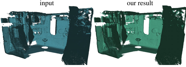
Figure 10: Large-scale denoising I: Our method exhibits good scalability in problem size: for an indoor scan with 1.15 million points, our denoising method takes 115s (convergence is reached in 5 iterations), with about 3s for local fitting and 20s for the global linear solve per iteration.
