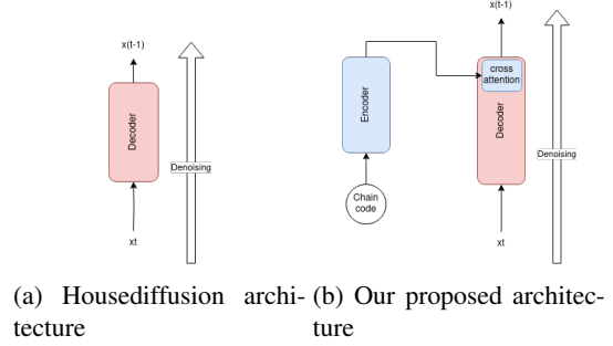
Figure 2: In both architectures, the diffusion denoising (from x_t to x_{t-1} ) is performed by the decoder, but unlike HouseDiffusion [29], we add a cross-attention module and an encoder to take into account constraints on partial shapes, which are encoded as chaincodes.
