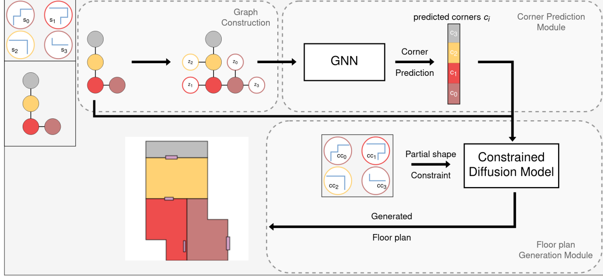
Figure 1: We consider for input the connectivity graph and a set of partial shapes associated to different rooms. The graph construction method attaches the Zernike Moments z_i = \text{Zernike}(s_i) to the corresponding room, for every partial shape s_i . We then compute the number of corners per room c_j thanks to our Graph Encoder. These information are then utilized as well as the Chain Code cc_i = \text{ChainCode}(s_i) to generate the corresponding floor plan. Each cc_i is used to condition the Constrained Diffusion Model that outputs the floor plan
