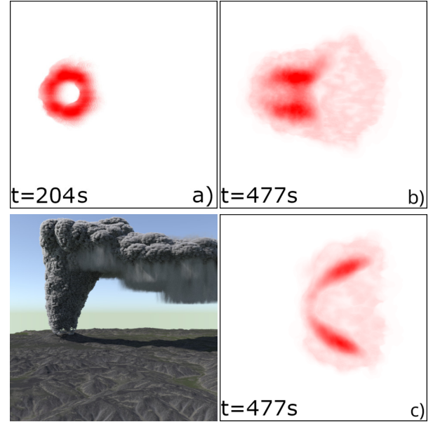
Figure 9: Ash fall density in the atmosphere under a wind from left to right, with darker red indicating greater density. a) Ash accumulated on the terrain before the formation of the umbrella; b) Ash in the top most layer below the umbrella, where most of the ash transfer takes place; c) Ash in the layer immediately below b).
