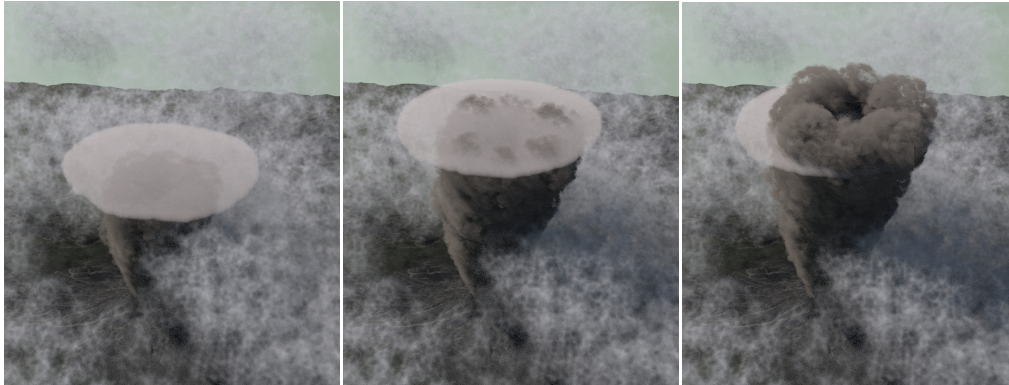
Figure 14: Cap cloud formation and absorption over a span of t = 30s .
