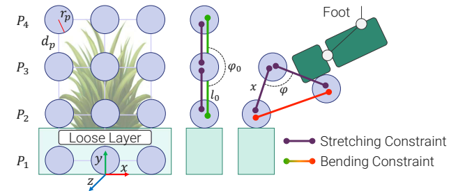
Fig. 5 A surface 2D plant-row model. Particles are vertically interconnected using stretching and bending constraints, enabling the model to retrieve its shape after trampling.
