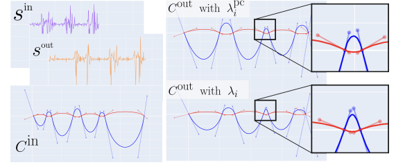
Figure 6: Semantic preserving time scaling applied to a smooth animation curve. The close-up view illustrates how our optimization helps to preserve the sharper curve of the second maxima already present in the initial animation and is associated with a dynamic change of direction.
