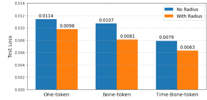
Figure 5: Results on Different Token Models.
