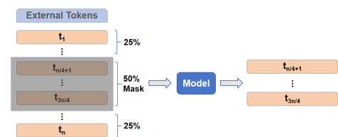
Figure 3: Model Framework.
