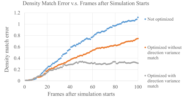
Figure 15: Density error for simulations before and after optimisation with and without direction variance error.
