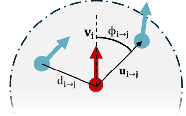
Figure 4: Perceptual terms: the distance to neighbour d_{i \rightarrow j} and bearing angle \phi_{i \rightarrow j} are defined by the relative position of the current agent a_i and its neighbour a_j .
