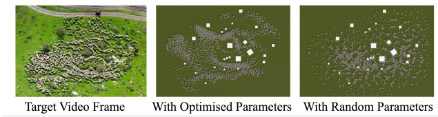
Figure 9: Simulation based on ‘sheep-broad’. [Left] Target video frame. [Middle] Learnt simulation. [Right] Simulation with random parameters before optimisation.
