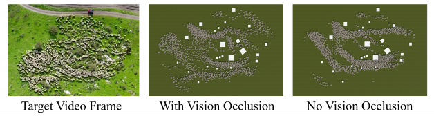
Figure 10: Assessing the impact of vision occlusion. [Left] A target video frame. [Middle] Learnt simulation with vision occlusion. [Right] Learnt simulation without vision occlusion.
