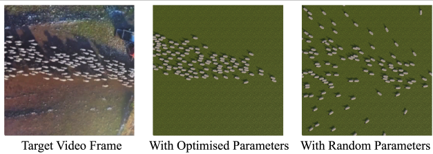
Figure 7: Simulation based on ‘sheep-narrow’. [Left] Target video frame. [Middle] Learnt simulation. [Right] Simulation with random parameters before optimisation.
