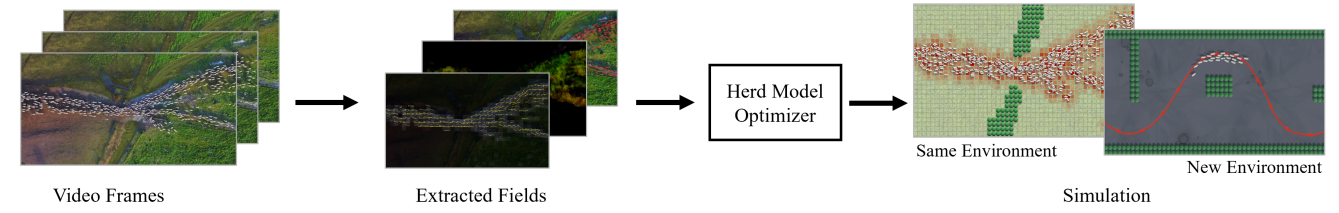
Figure 2: Learning and authoring pipeline. Starting with frames from video clips, grid-based density and velocity fields are extracted. This data is used to optimise our herd model with perception-related force parameters. Finally, the learnt herd can be deployed either in an environment that matches the source clip or a new user-defined environment.
