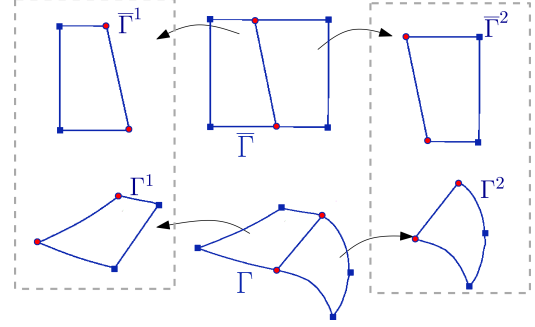
Figure 1: Recursive subdivision step: the 2D pattern and the corresponding 3D contour (middle) are split into two pieces (left and right) along a fold line, which is straight in pattern space.
